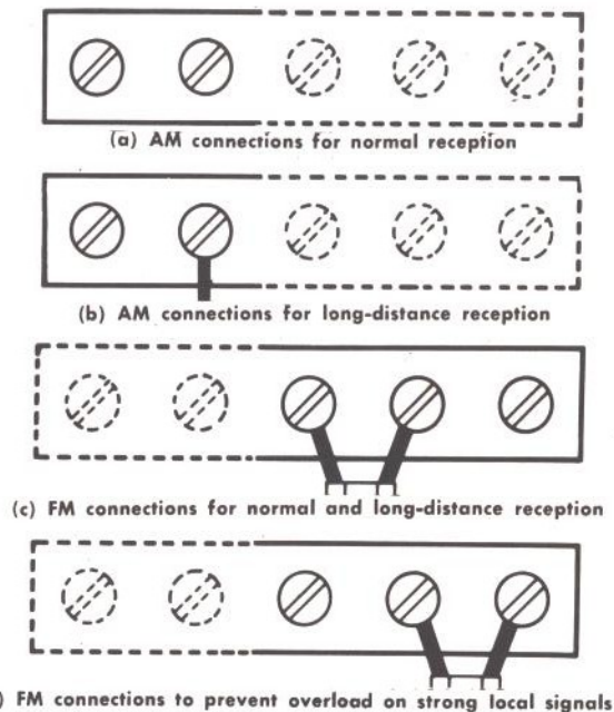
(d) FM connections to prevent overload on strong local signals FIGURE 2. Antenna connections.
